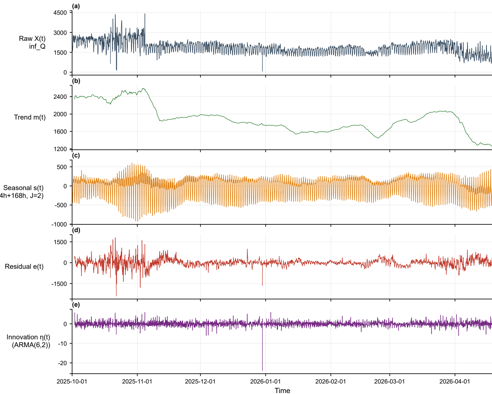
Multi-scale decomposition — inf_Q (influent, hour) [2025-10-01~2026-04-19]
